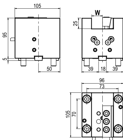
TIPO - TYPE Stelo quadro assiale Axial face and cutting holder
